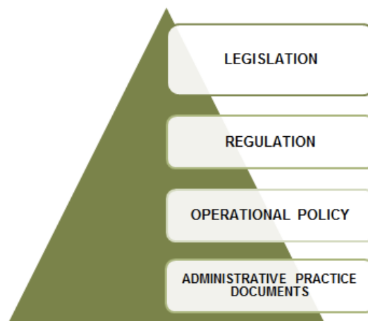
Figure 9: Hierarchy of policy instruments
