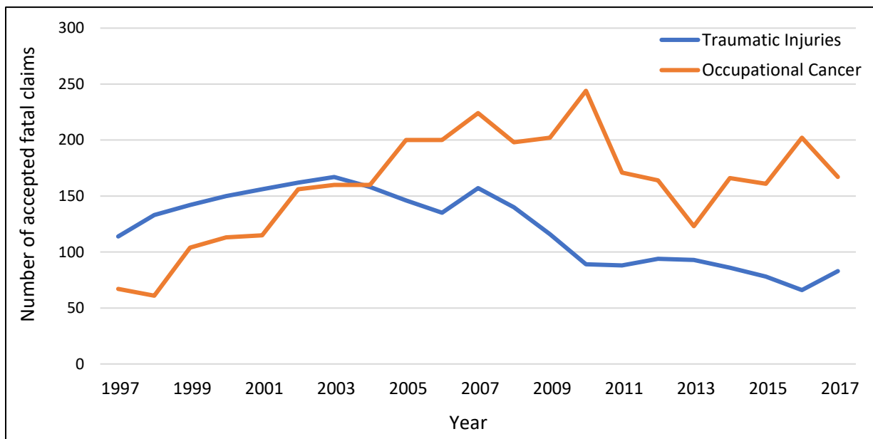
Figure 2: WSIB accepted workplace fatalities (1997–2017)
